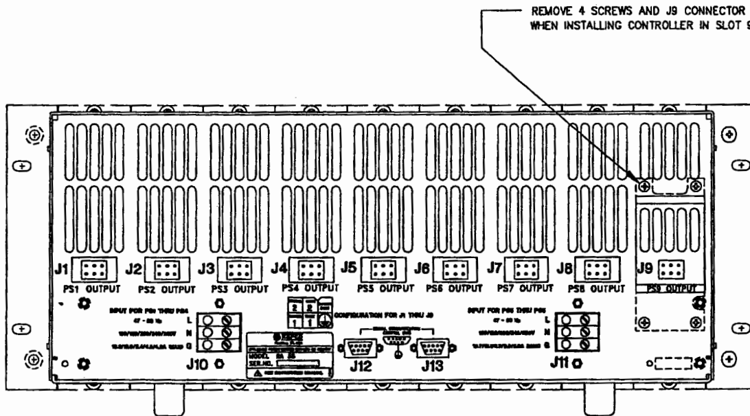
FIGURE 2. RA 55 BACKPLATE ASSEMBLY
